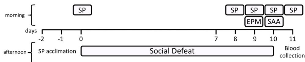
Fig. 1. Experimental design. Timeline showing all the steps of the experimental manipulations. Thirty-day-old C57BL/6 male mice were exposed daily to chronic defeat stress (CSDS) from an aggressive CD-1 mouse during 5 min of physical interaction (occurring in the afternoons), followed by 24 h of protected cohabitation with the aggressor (threat period) over 10 days.
